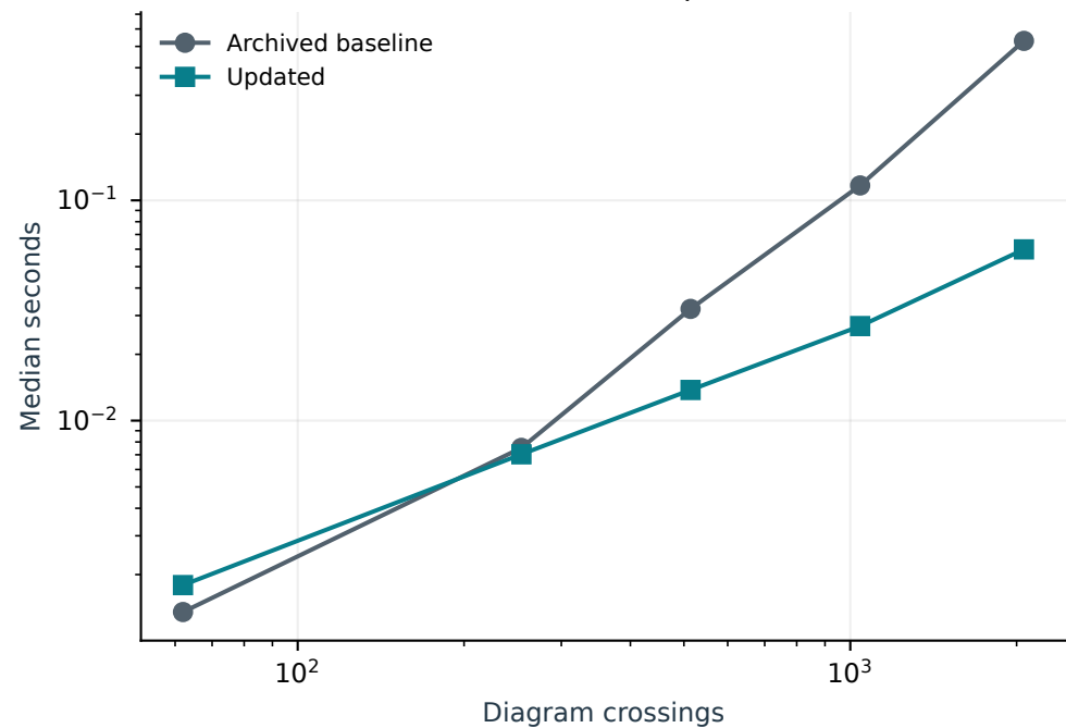
Alexander filter, forced sparse backend
