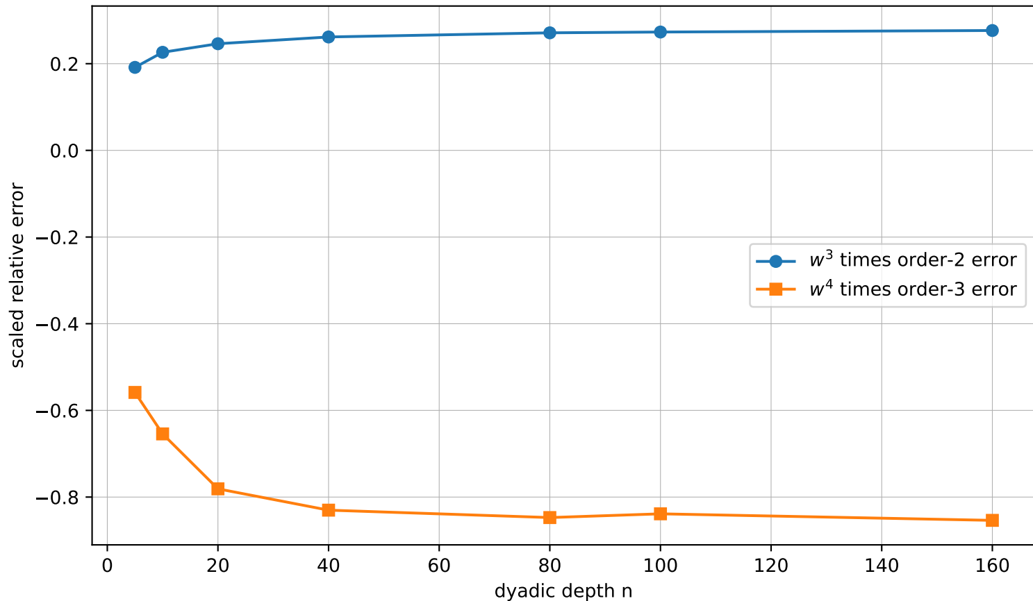
Stabilization of the first omitted W-resummed coefficients
