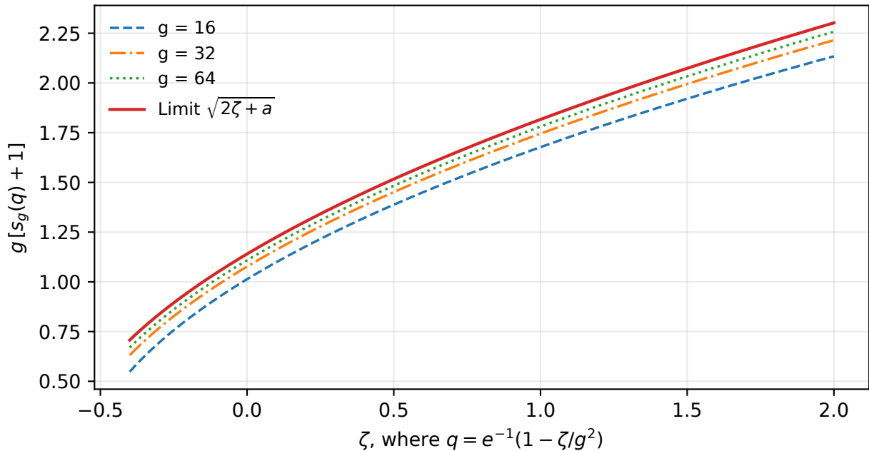
Curvature-shifted inner limit: a = 1.3 , b = 0.7
