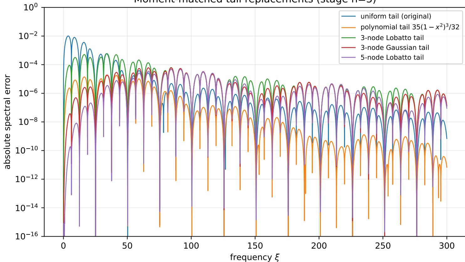
Moment-matched tail replacements (stage n=3)
