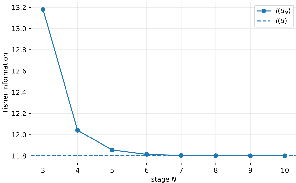
Fisher information under successive uniform convolutions
