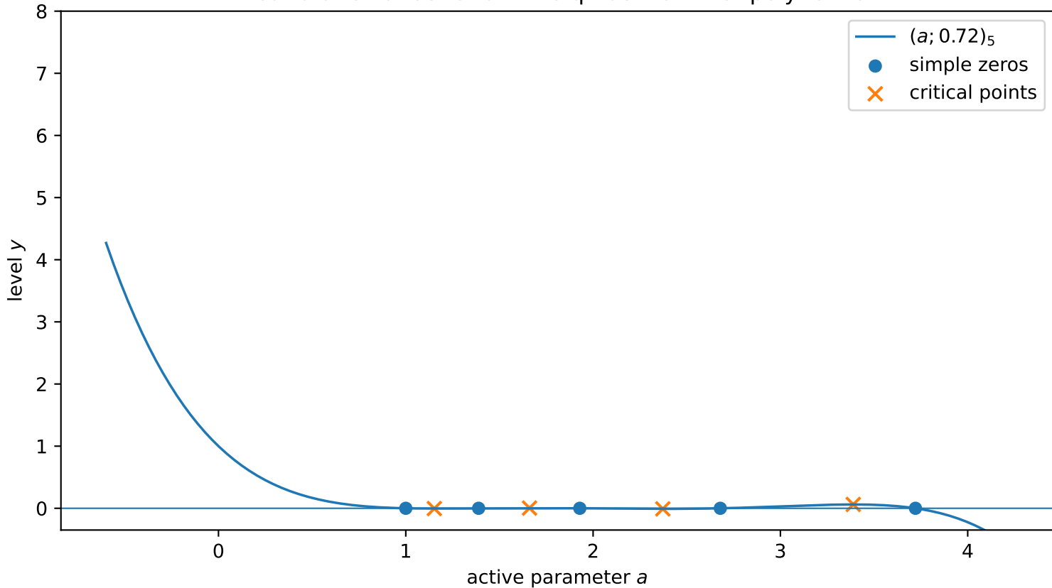
Real branch atlas for a finite q-Pochhammer polynomial
