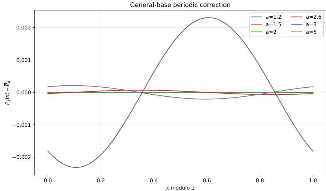
Figure 4: Centered periodic corrections P_a - \overline{P}_a . The dyadic oscillation is small but nonzero; its amplitude grows substantially for the displayed larger bases.
