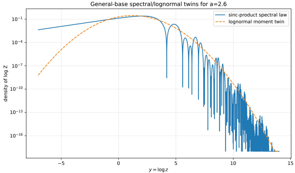
Figure 6: Log-frequency densities of the sinc-product spectral law and its lognormal moment twin for a = 2.6 . Their moments agree exactly, while the spectral density retains the visible zero and oscillation structure forced by the sinc factors.
