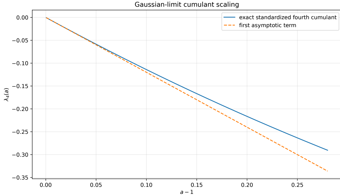
Figure 5: The exact standardized fourth cumulant and its first asymptotic term.
