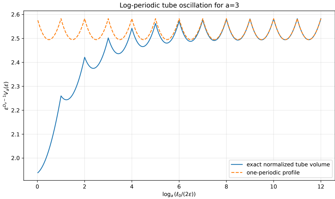
Figure 2: The exact normalized tube volume for a = 3 . The approach to a nonconstant one-periodic profile verifies the lattice oscillation in theorem 6.2 .
