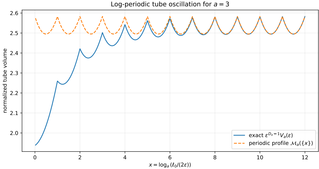
Figure 2: The exact normalized tube volume for a = 3 . The approach to a nonconstant one-periodic profile verifies the lattice oscillation in theorem 6.2 .
