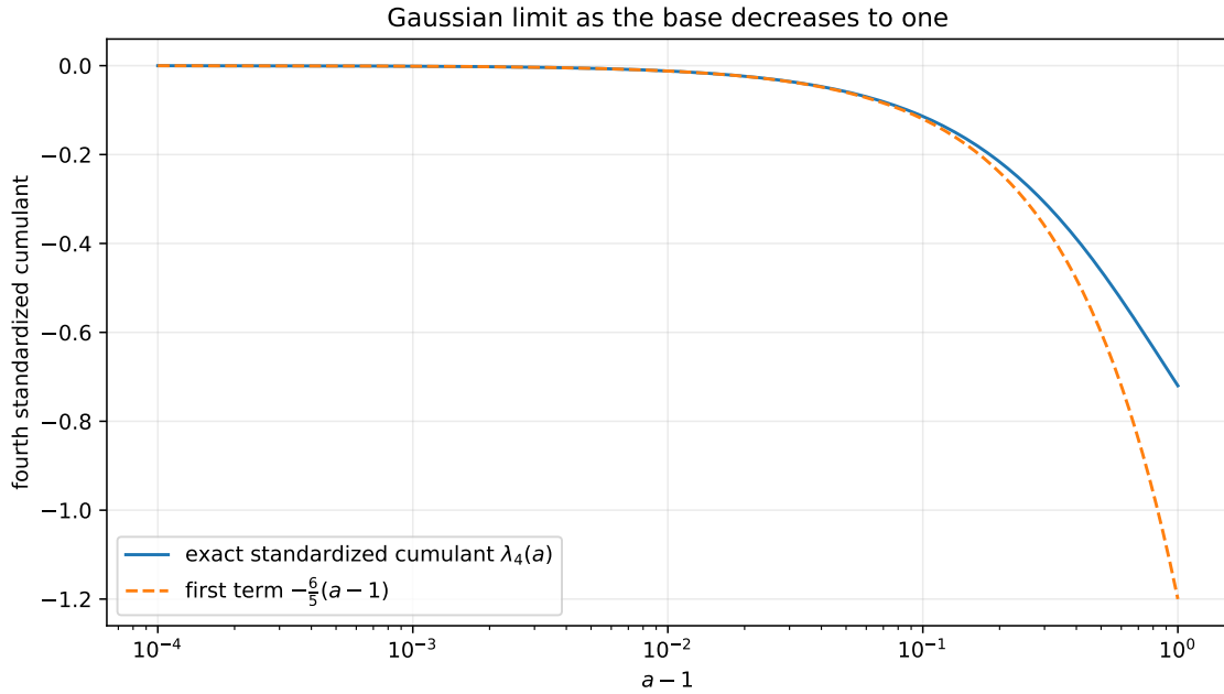
Figure 6: The exact standardized fourth cumulant and its first asymptotic term.
