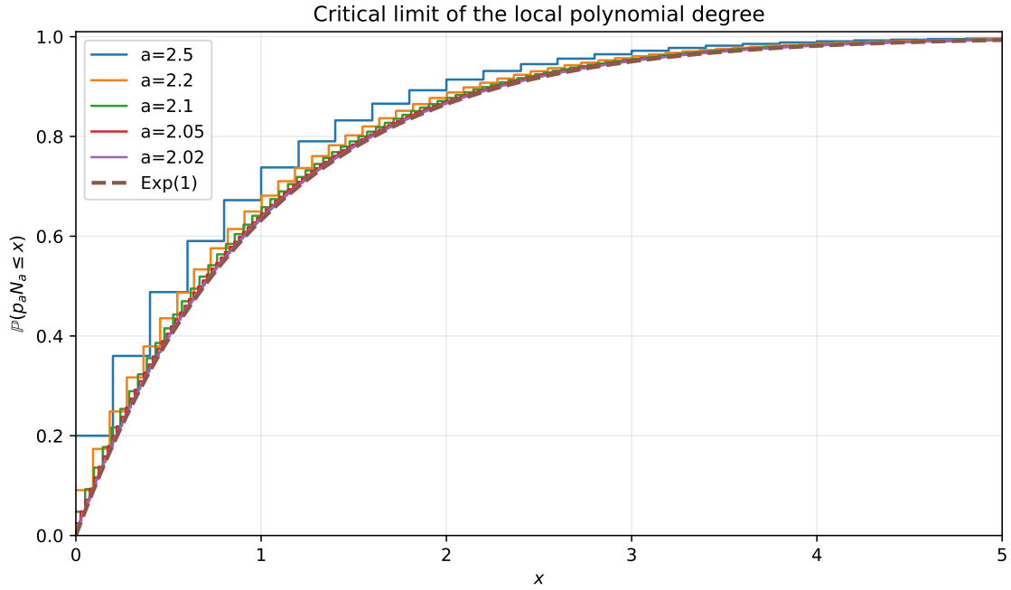
Figure 3: Distribution functions of p_a N_a approaching 1 - e^{-x} as a \downarrow 2 .
