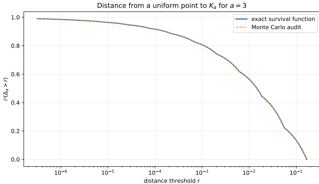
Figure 4: Exact and simulated survival functions of \Delta_a = \text{dist}(Q_a, K_a) for a = 3 . The visible changes of scale occur when the threshold crosses half the length of a gap generation. The corresponding Mellin moments are audited in data/distance_validation_a_3.csv .
