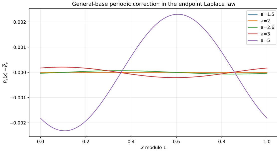
Figure 5: Centered periodic corrections P_a - \bar{P}_a . The dyadic oscillation is small but nonzero; its amplitude grows substantially for the displayed larger bases.
