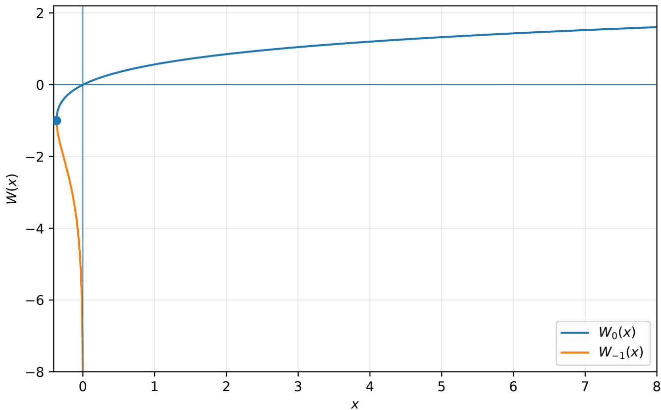
The two real branches of the Lambert W function
