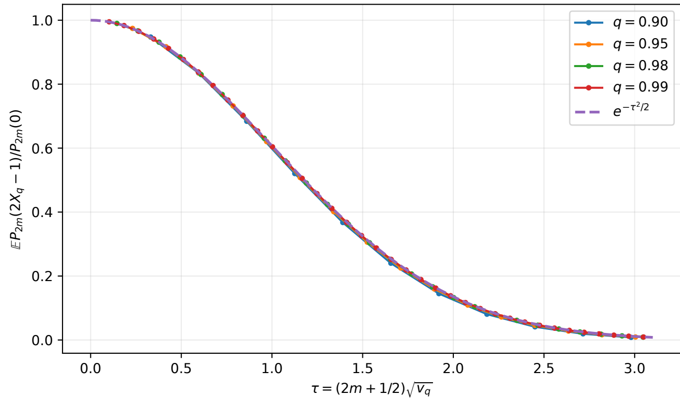
Legendre heat-kernel double scaling
