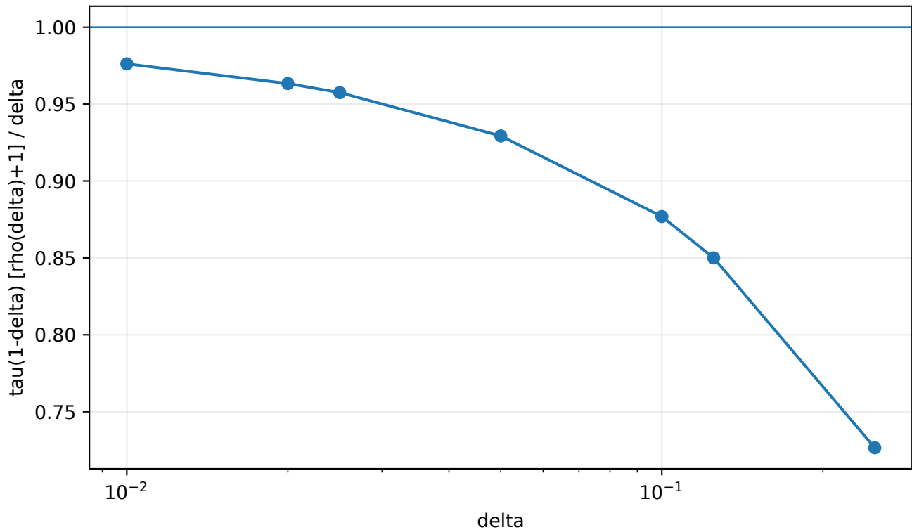
Endpoint Stein-kernel asymptotic diagnostic
