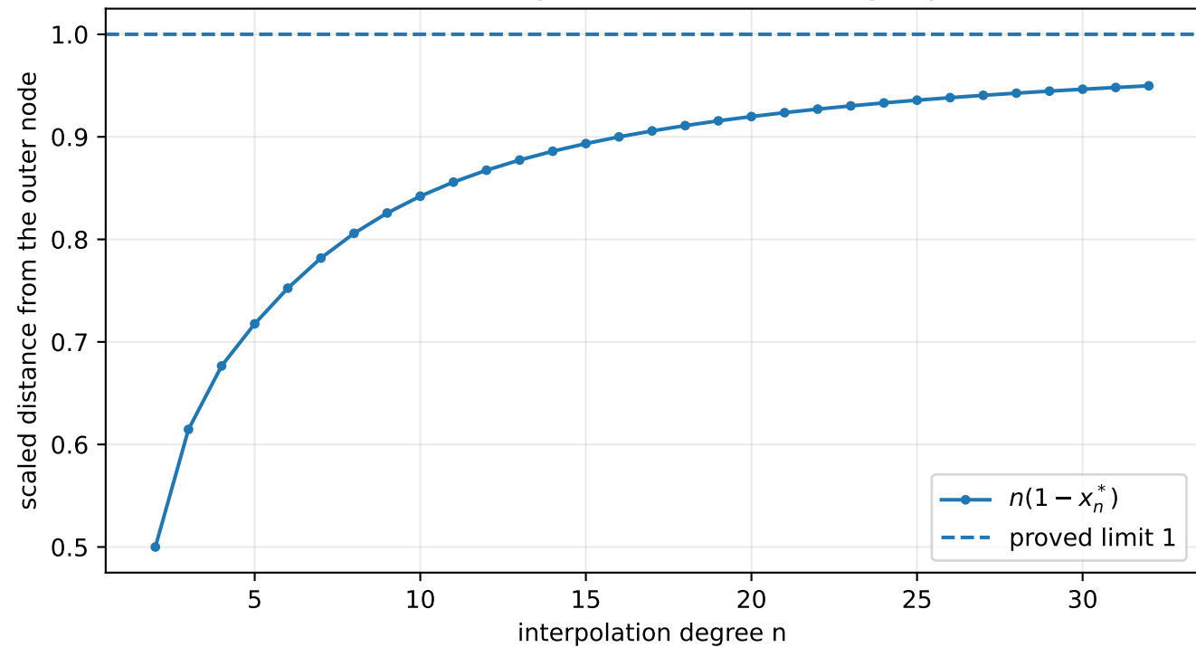
Location of the geometric-comb Lebesgue peak
