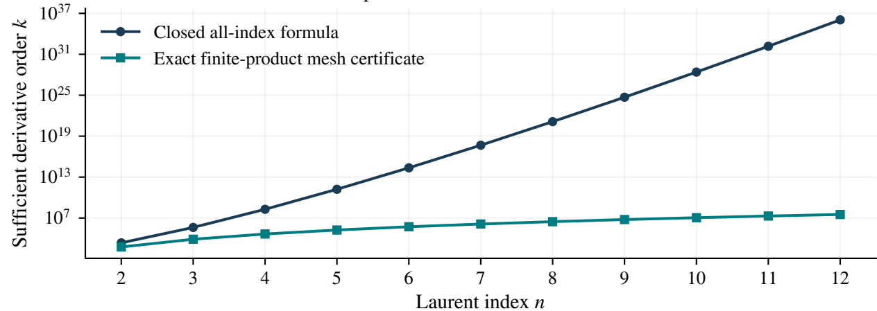
Two proved uniform saturation bounds
