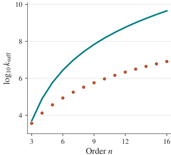
(b) Finite certificates: 3 \leq n \leq 16
