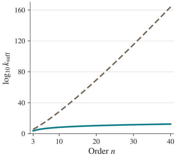
(a) General bounds: 3 \leq n \leq 40
