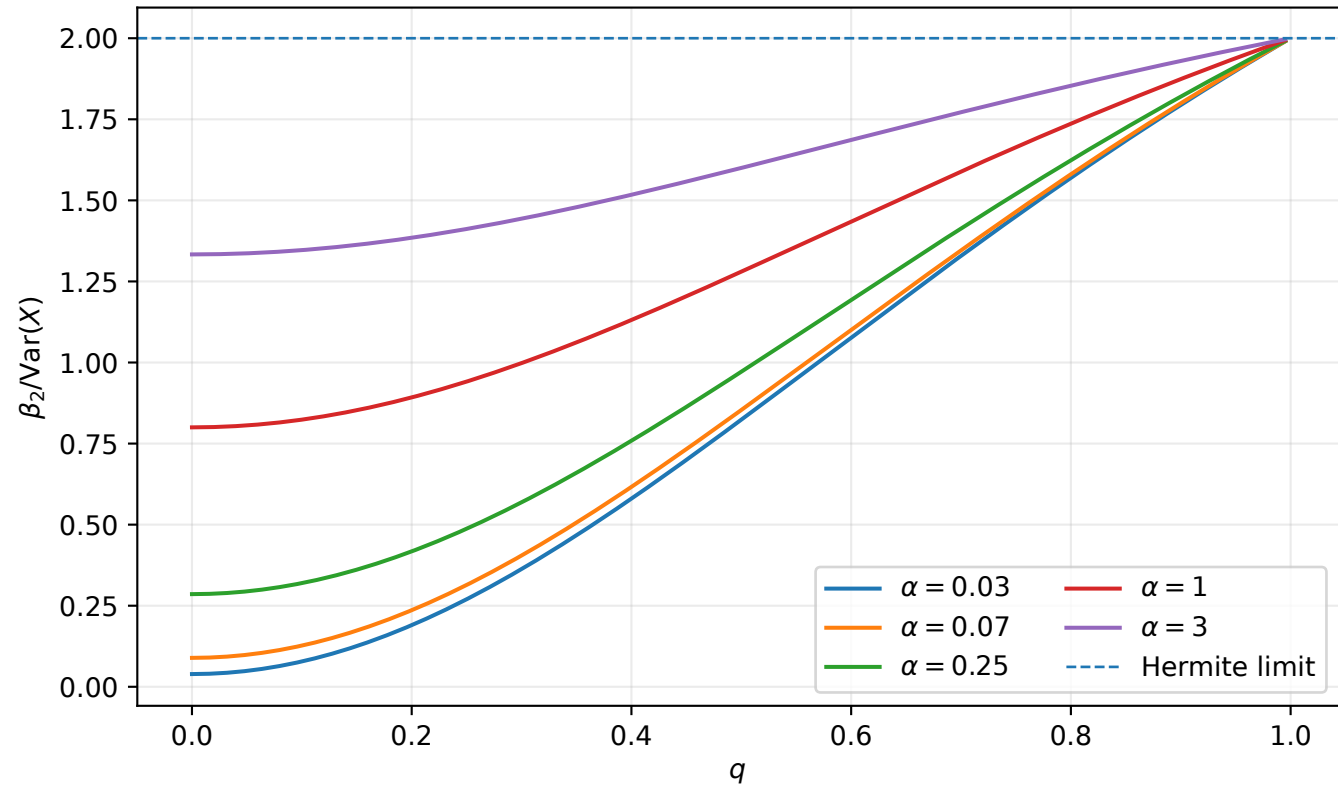
Second monic recurrence coefficient: exact monotone flow
