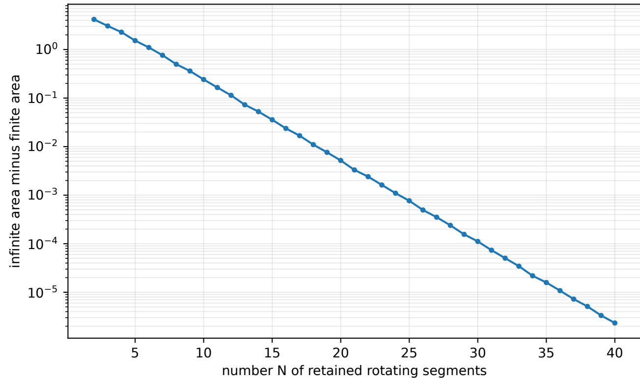
Geometric convergence of rotating-zonotope area
