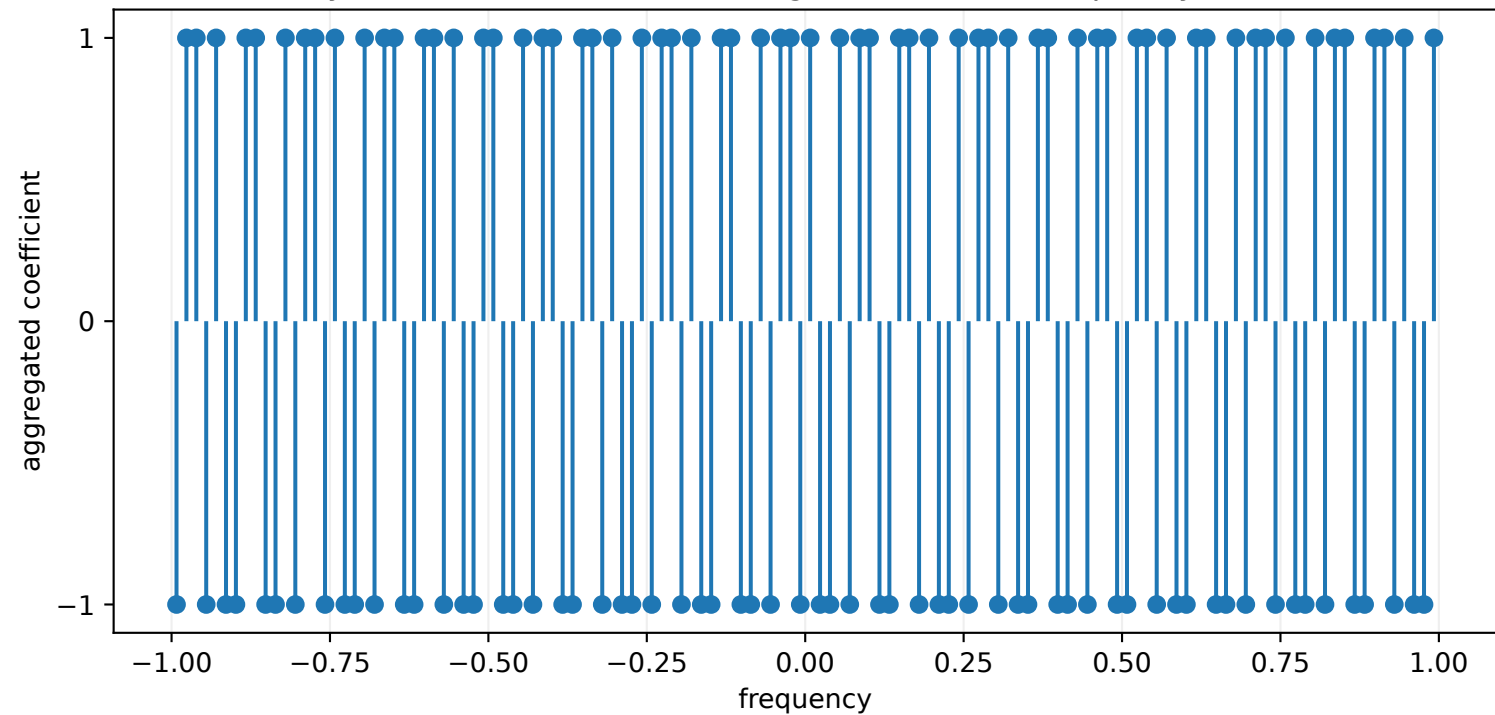
Dyadic level 7: Thue--Morse signs on the odd frequency lattice
