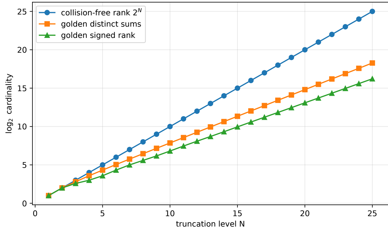
Holonomic rank and exact-overlap compression
