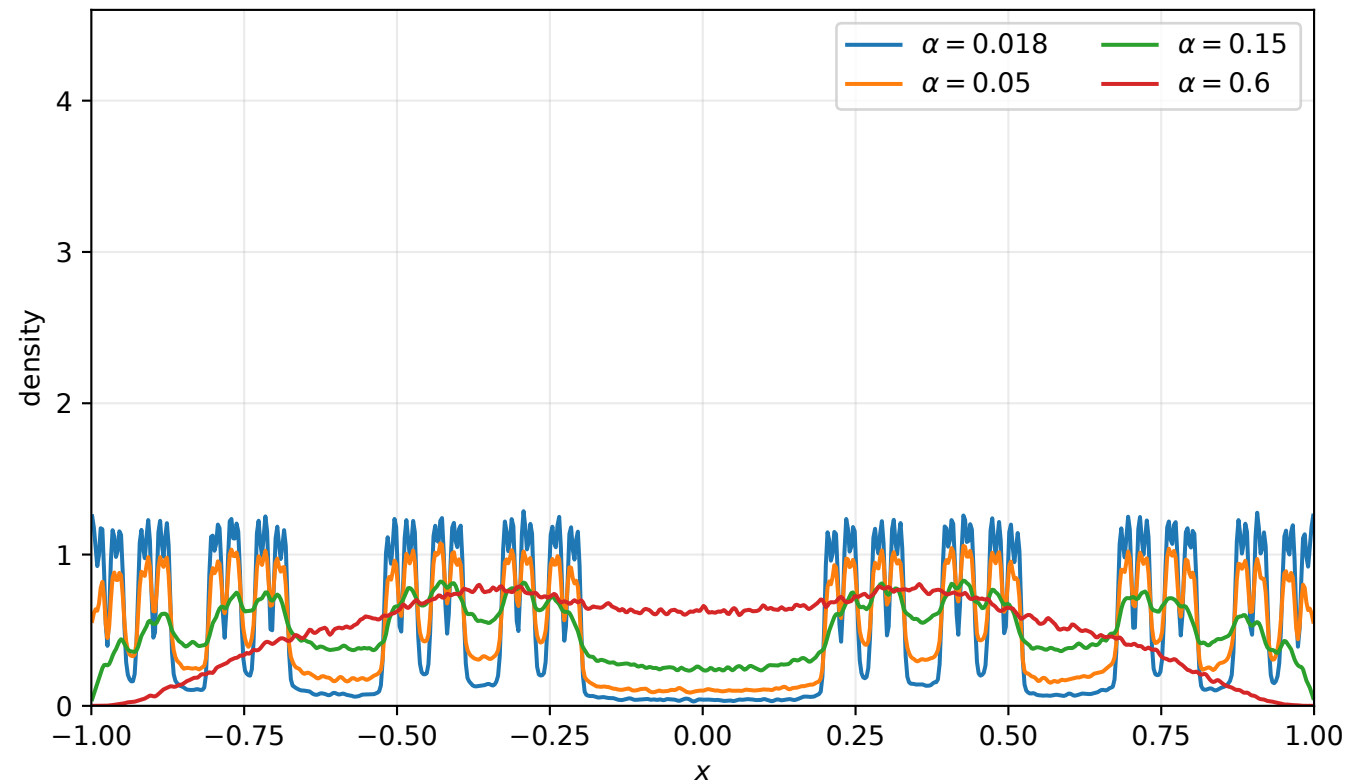
Smooth desingularization of the q = 0.4 Bernoulli convolution
