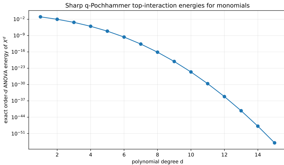
Figure 3: The exact highest-order interaction energy (69). The quadratic exponent in the dyadic factor forces superexponential decay even after multiplication by (d!)^2 .
