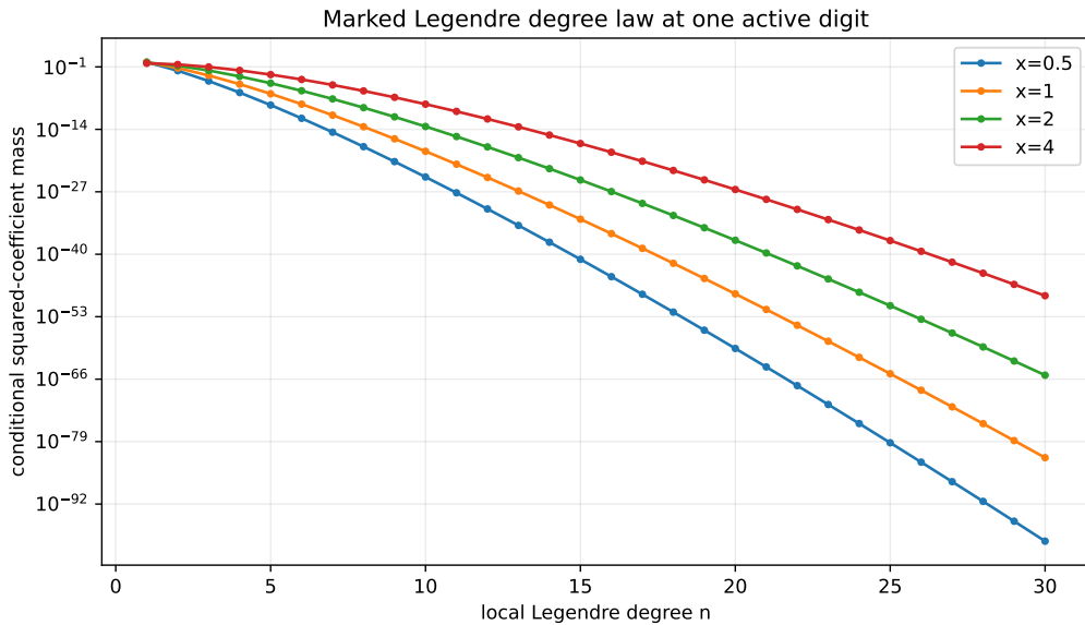
Figure 2: The local degree mark in (52). Larger local field x activates higher Legendre degrees, while the far dyadic tail remains almost entirely degree one when it activates.
