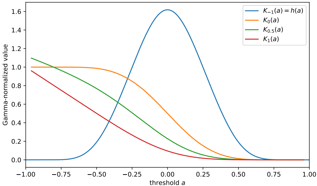
Difference-distribution order ladder
