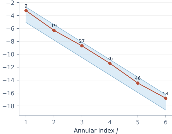
Roots 3/10 \pm 2i/5
