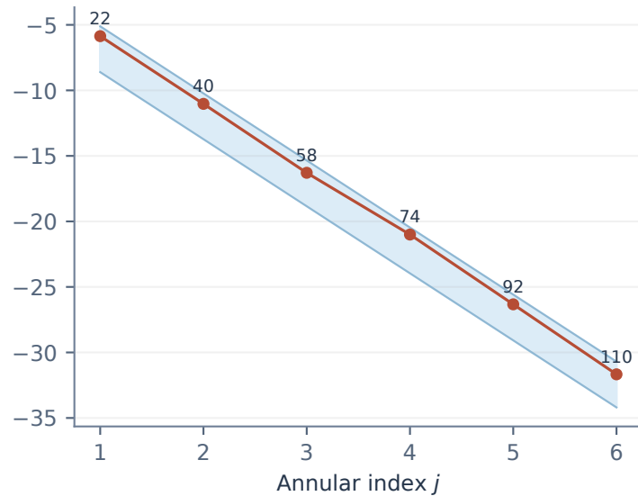
Repeated complex roots
