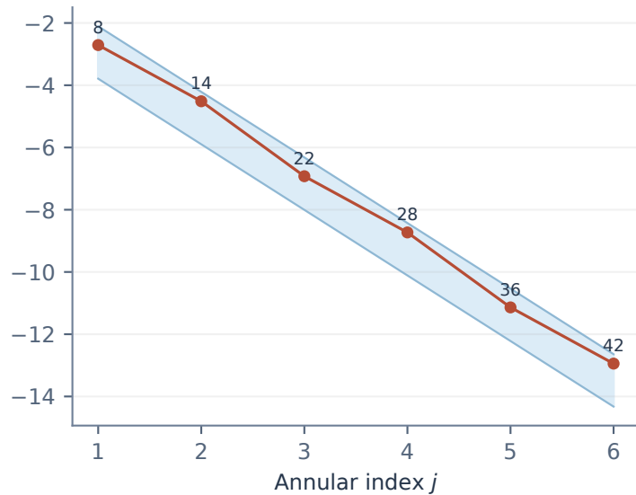
Complex roots; exact zeros
