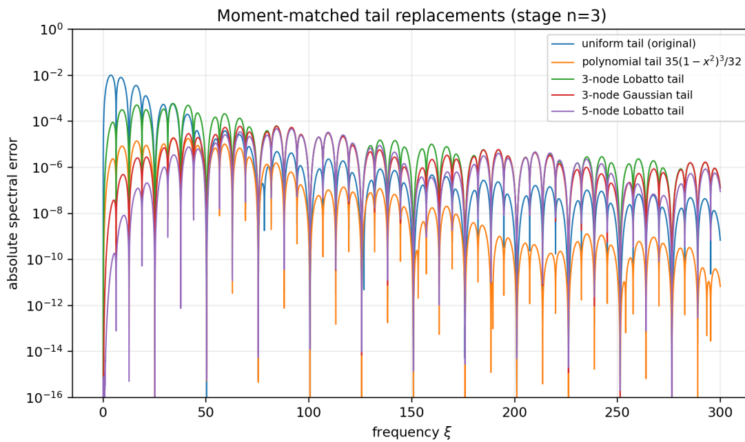
Figure 12: Absolute Fourier errors of the closure menu at stage n = 3 ; the faster rates are visible over most of the frequency range, with leading profiles attaining maxima on progressively more distant lobes.
