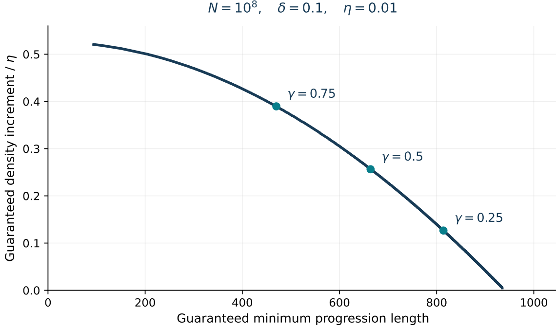
Figure I.24.1: The proved density–length tradeoff, evaluated at fixed N = 10^8 , \delta = 0.1 , and normalized correlation \eta = 0.01 . The vertical axis divides the guaranteed increment by \eta . These points are evaluations of formulas, conditional on the correlation hypothesis, rather than measurements of extremal sets.
