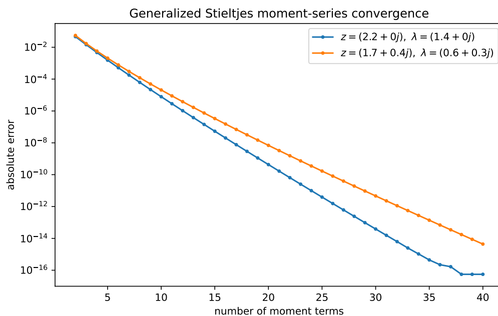
Figure 12: Convergence of the exact-moment expansion (1495) at two real/complex parameter pairs.
