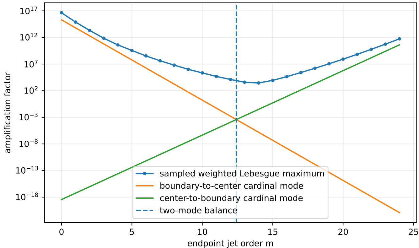
Conditioning at N=64: two opposing endpoint modes
