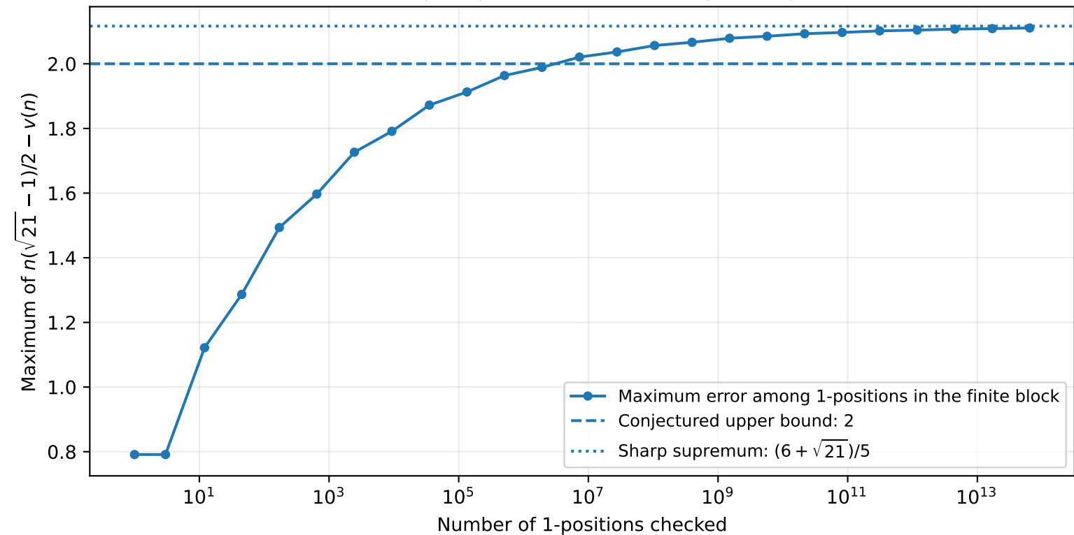
A small discrepancy that exceeds 2 only at large indices
