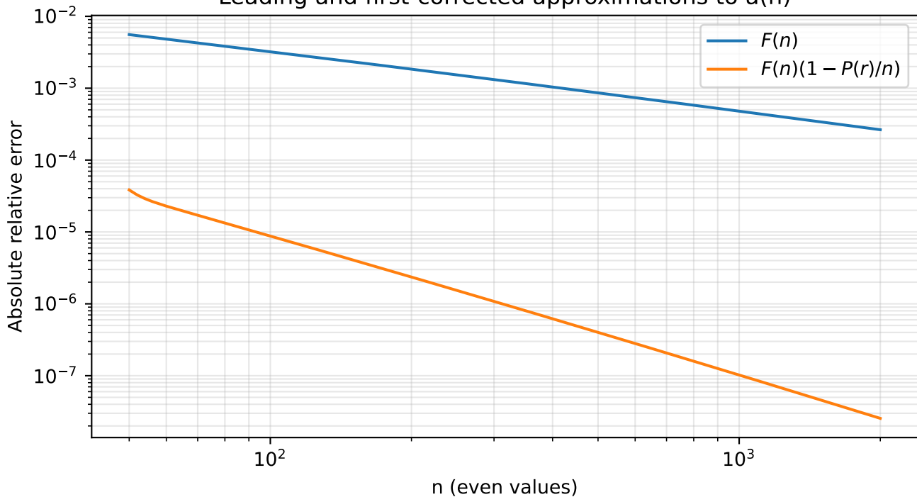
Leading and first-corrected approximations to a(n)
