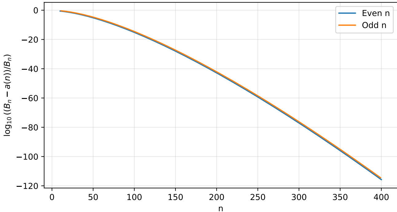
The relative contribution of the omitted partitions
