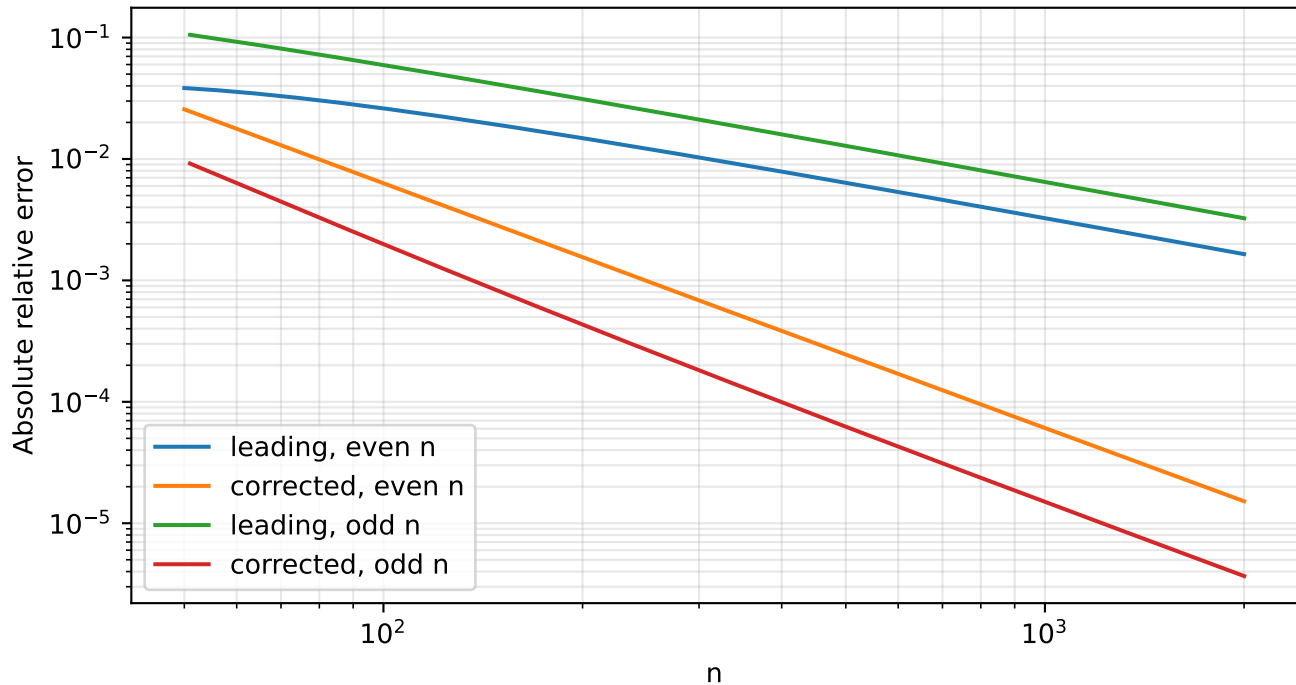
Parity-sensitive approximations to the omitted tail
