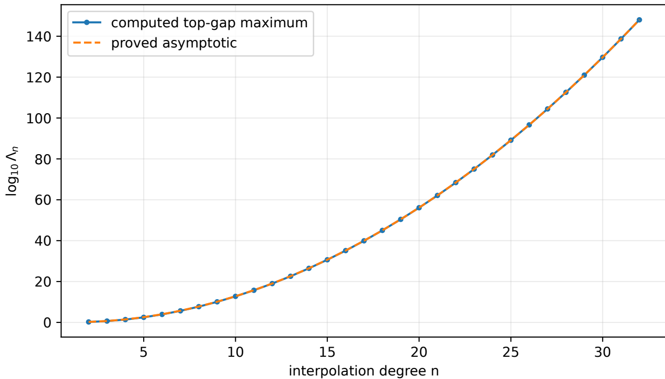
Lebesgue growth for the half-base comb 1, 2^{-1}, \dots, 2^{-n}
