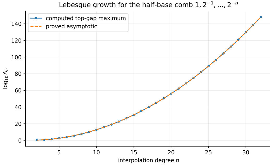
Figure 12.1: Top-gap maxima and the sharp global asymptotic 2(-q; q)_{\infty} q^{-\binom{n}{2}} / (en) for q = 1/2 . Logarithmic arithmetic is essential: the ordinate already exceeds 10^{148} at n = 32 .
