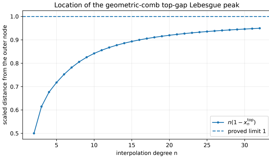
Figure 12.2: The scaled top-gap location n(1 - x_n^{\text{top}}) . The limiting value 1 is the maximizer of \alpha e^{-\alpha} in Theorem 7.2.
