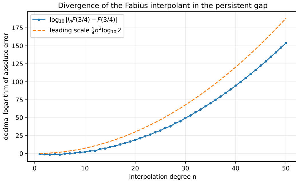
Figure 12.3: Exact-rational Fabius interpolation error at x = 3/4 . The plotted quadratic comparison is the leading n^2/4 term suggested by Conjecture 10.6 ; the negative (n/2) \log n correction is visible as a substantial downward displacement.
