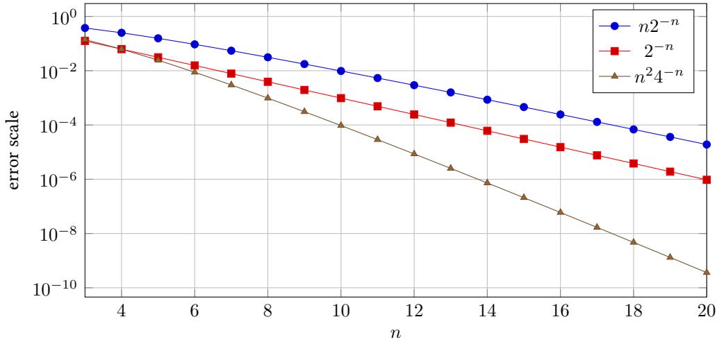
Figure 4: The three scales in (634). The deterministic center drift n2^{-n} dominates the one-cell scale 2^{-n} and the quadratic Taylor scale n^2 4^{-n} .
