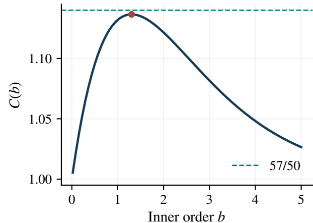
Sharp constants at fixed inner order
