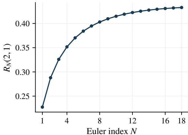
Scaled errors need not decrease
