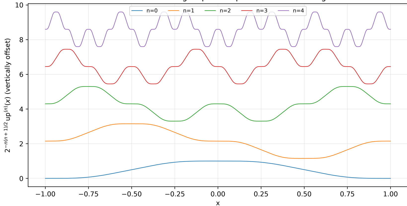
Exact derivative tiling: copies of up with Thue--Morse signs
