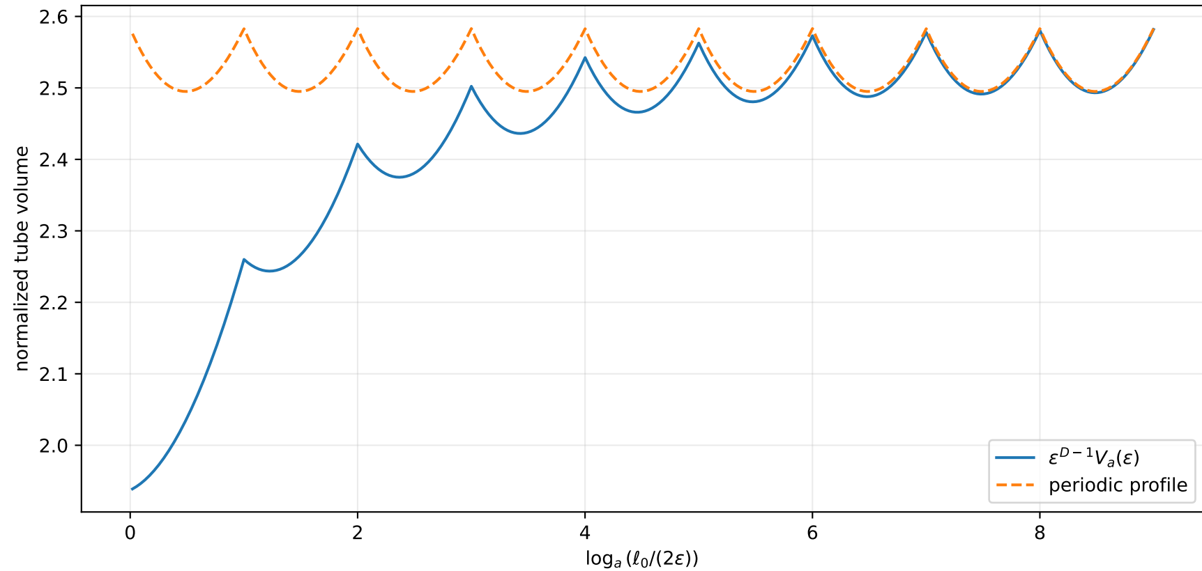
Exact logarithmic tube oscillation for a = 3
