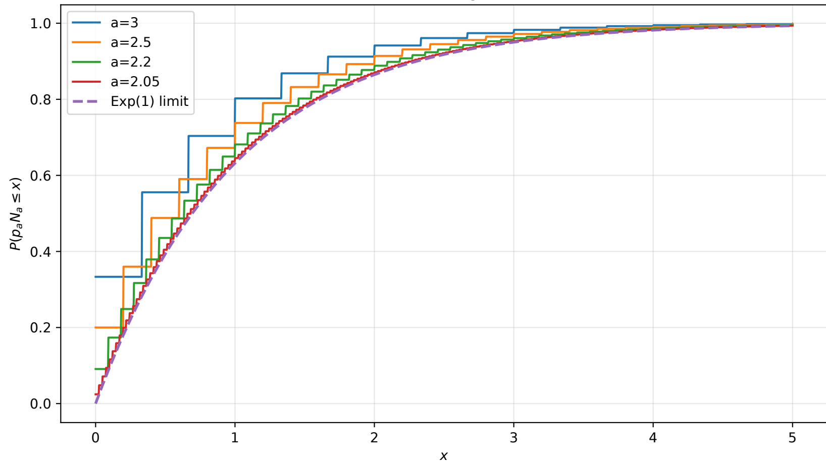
Critical local-degree limit
