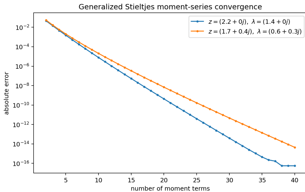
Figure 12: Convergence of the exact-moment expansion (1505) at two real/complex parameter pairs.
