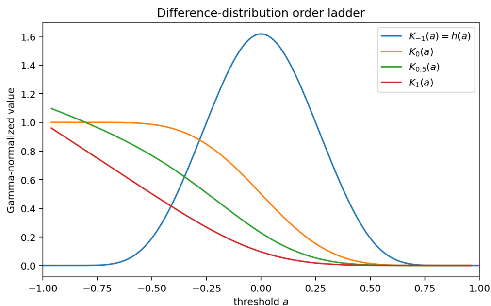
Figure 13: Several real-order slices of the entire difference hierarchy. The order -1 slice is the difference density, order 0 is its tail, and positive orders are fractional positive-part integrals.
