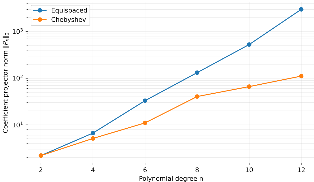
Obliquity of the exact coefficient-space projector
