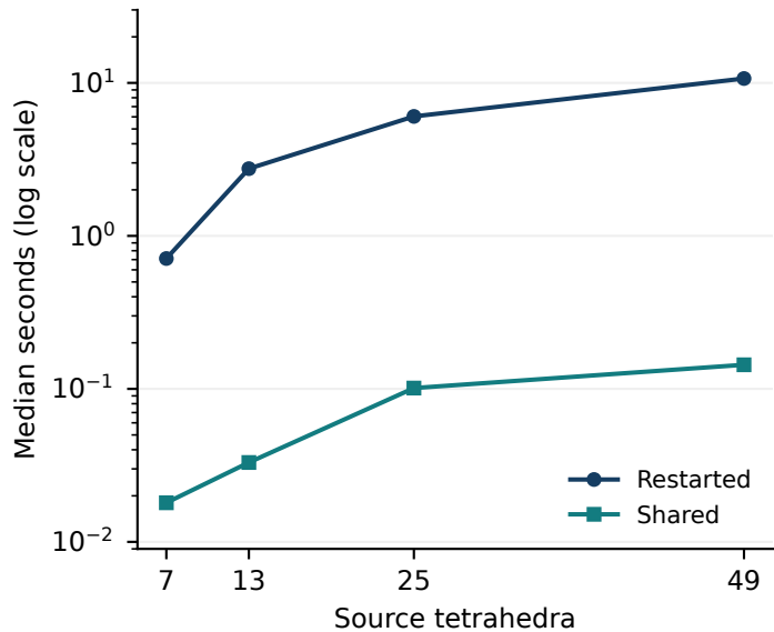
First verified strict descent
