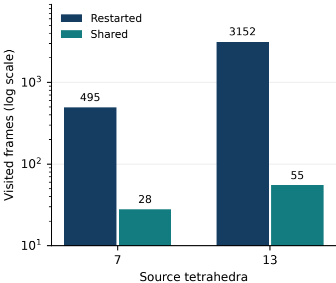
Complete covered-family search
