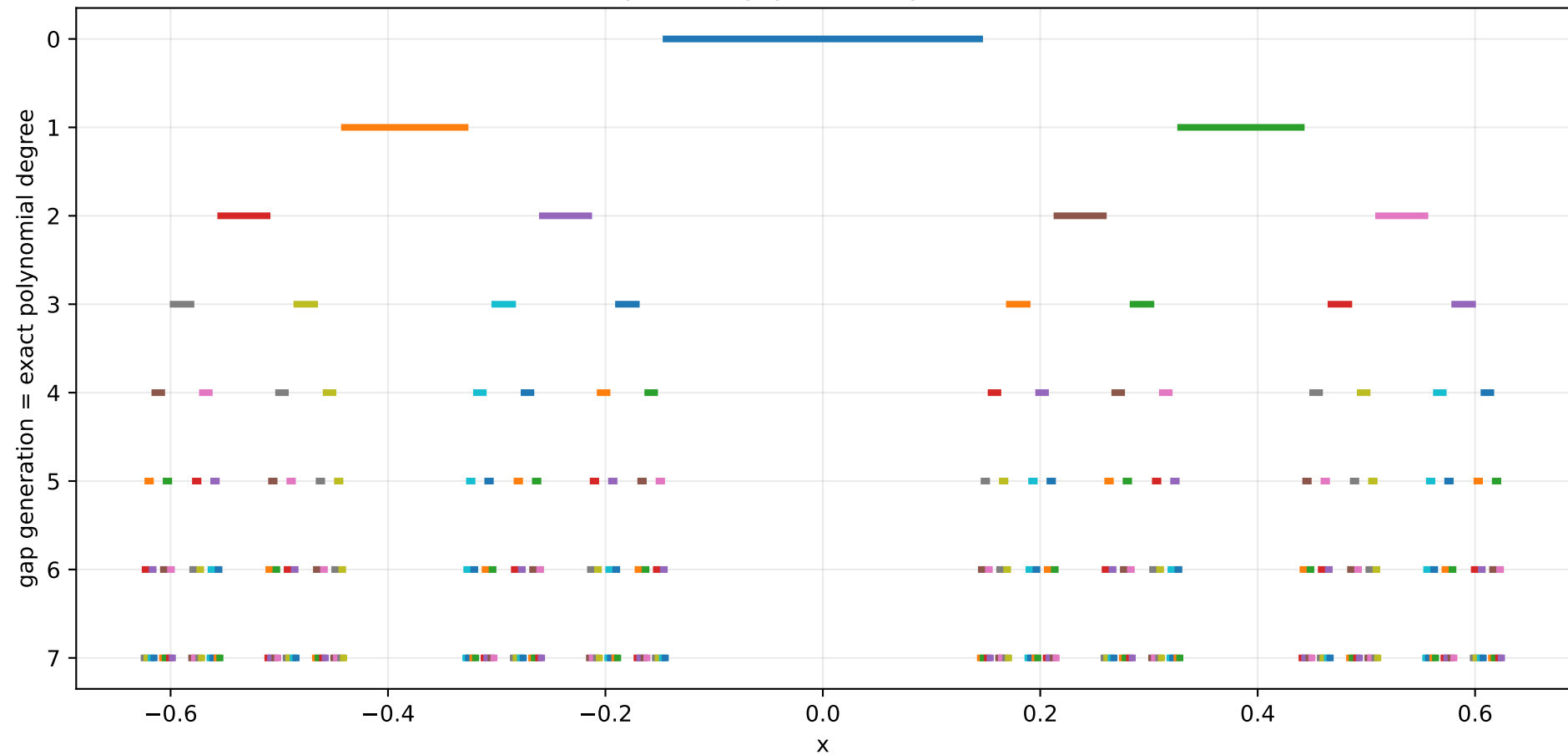
Polynomial-gap hierarchy for a=2.6
