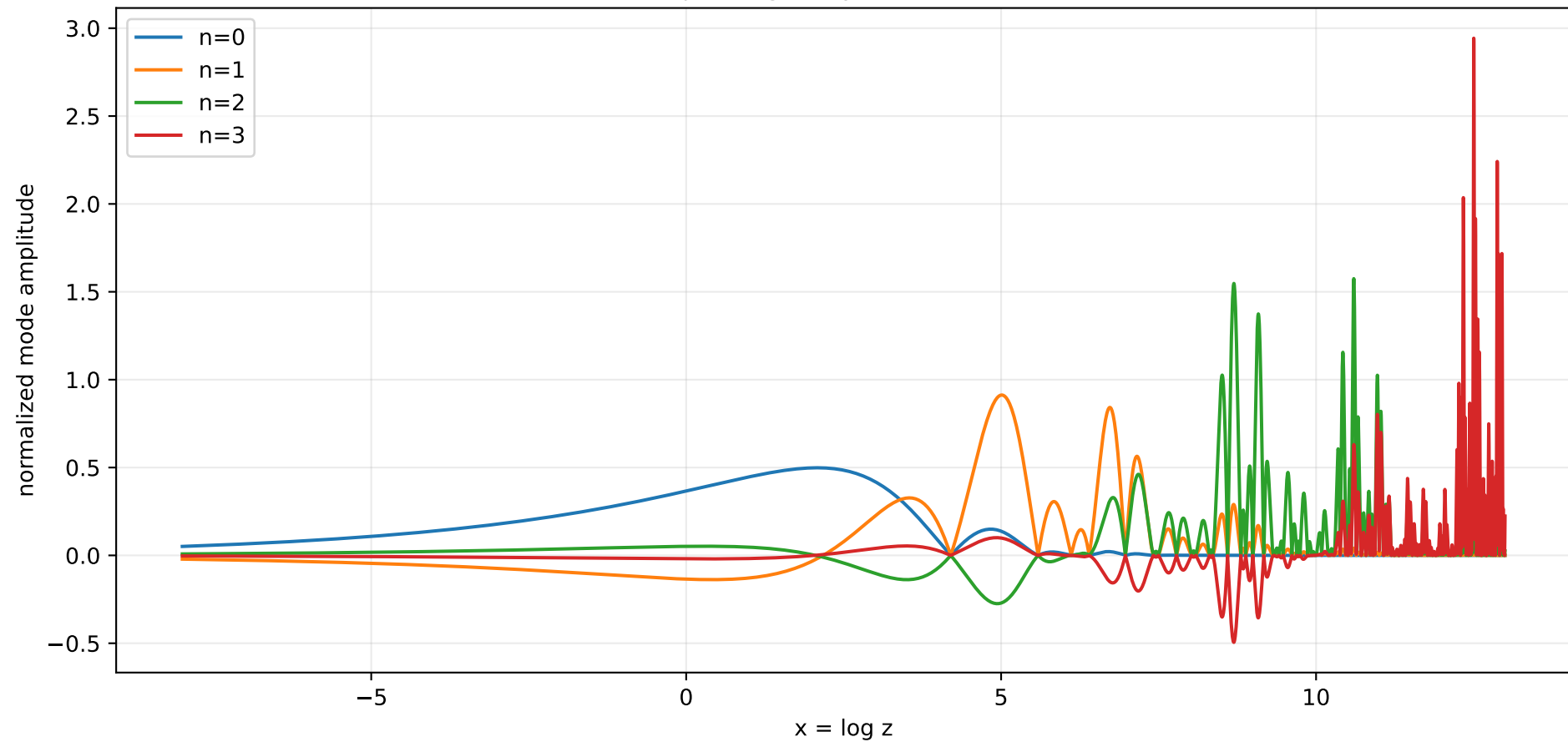
Scaled Stieltjes-Wigert spectral modes for a=2.6
