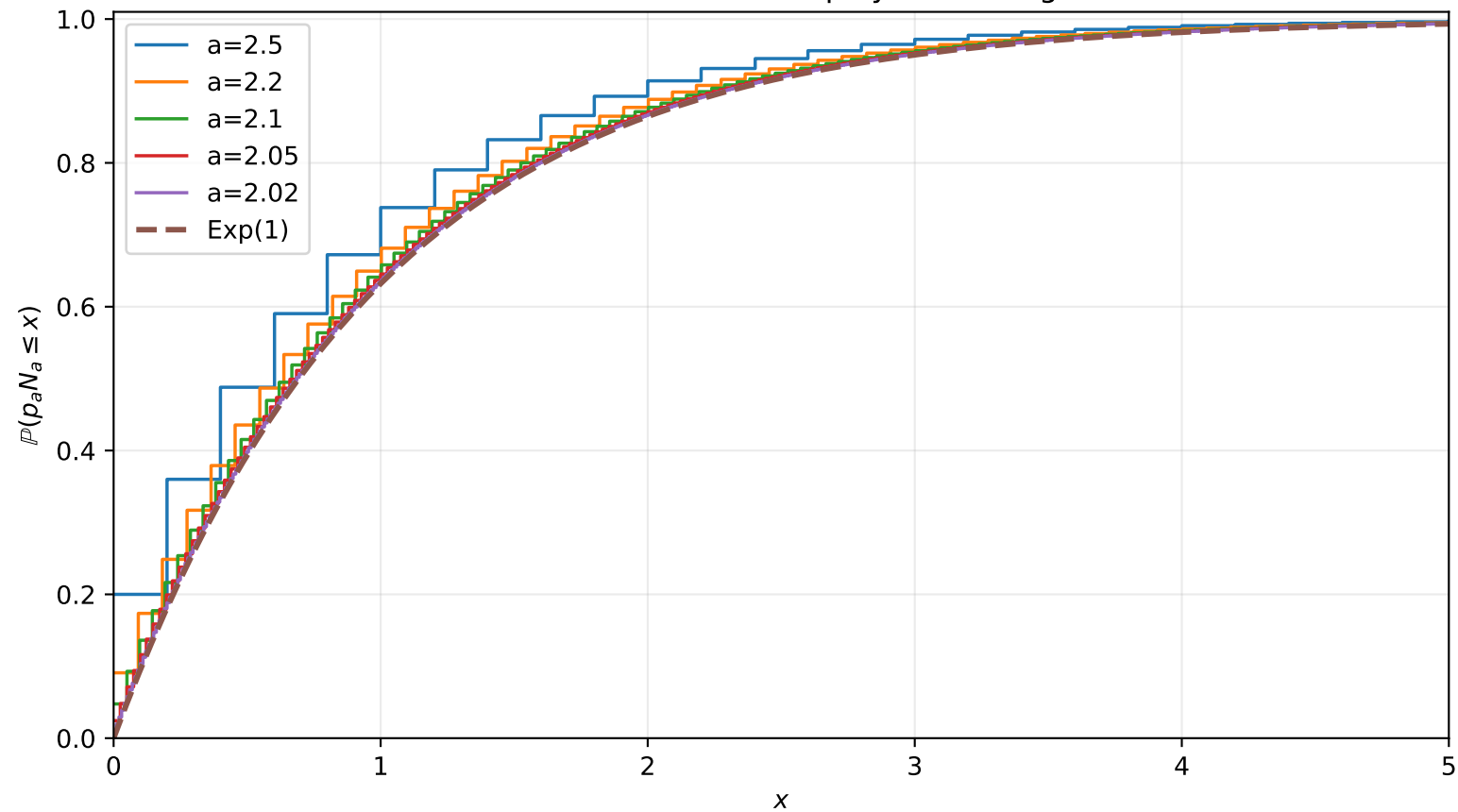
Critical limit of the local polynomial degree
