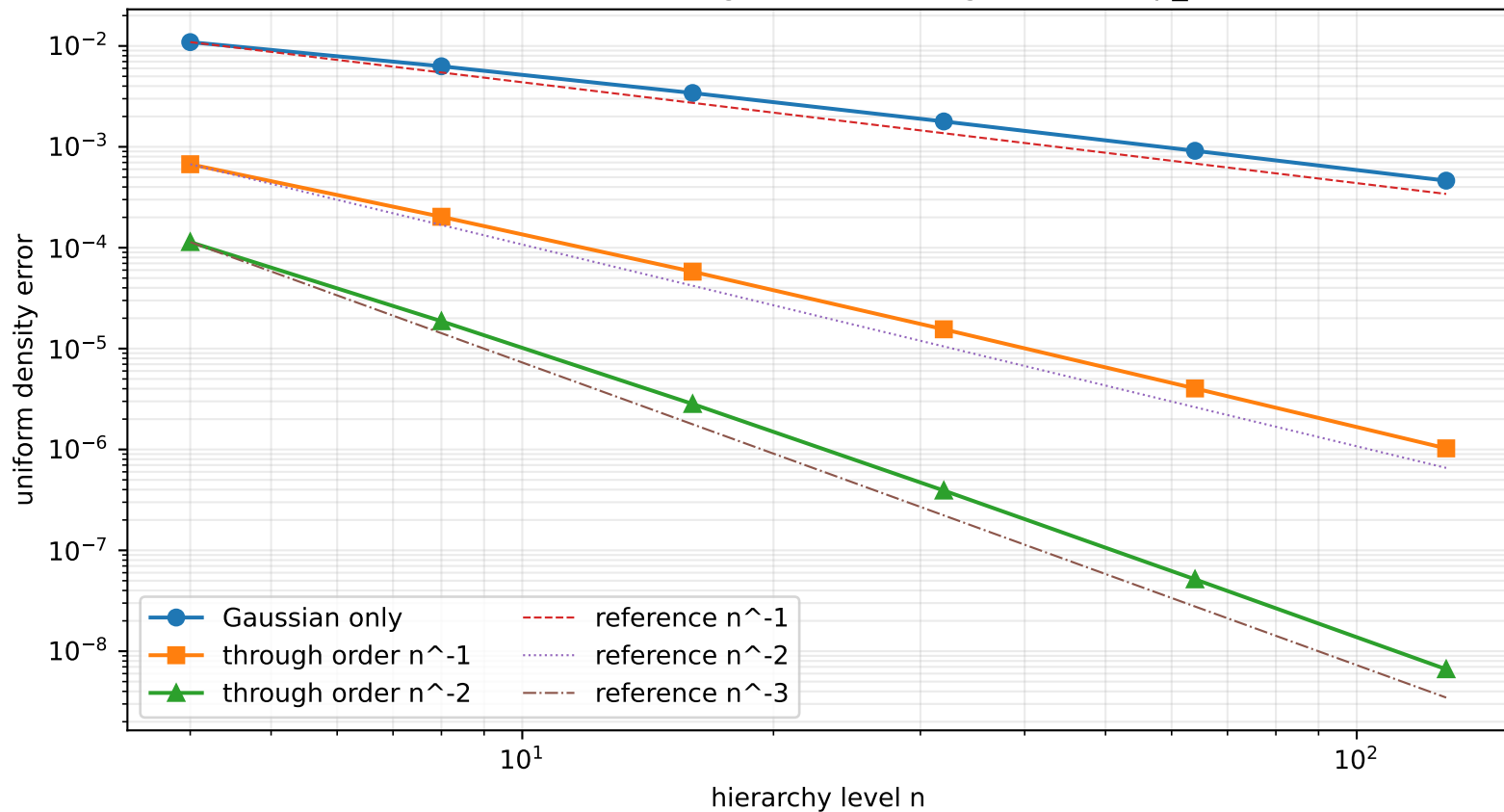
Exact-cumulant Edgeworth convergence for Fup_n
