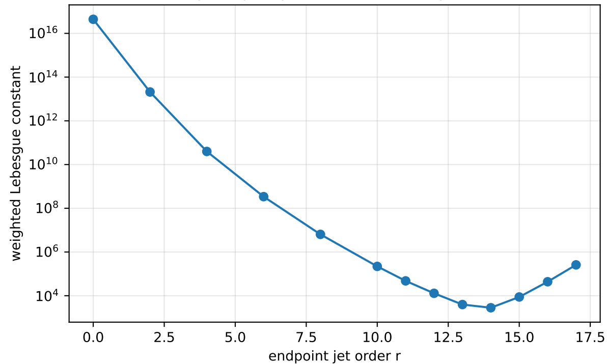
Endpoint-jet operator conditioning, N=64
