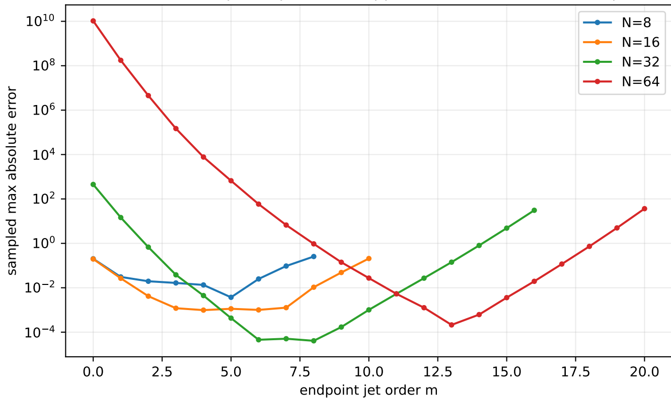
Rvachev bump interpolation: suppression and reverse blow-up
