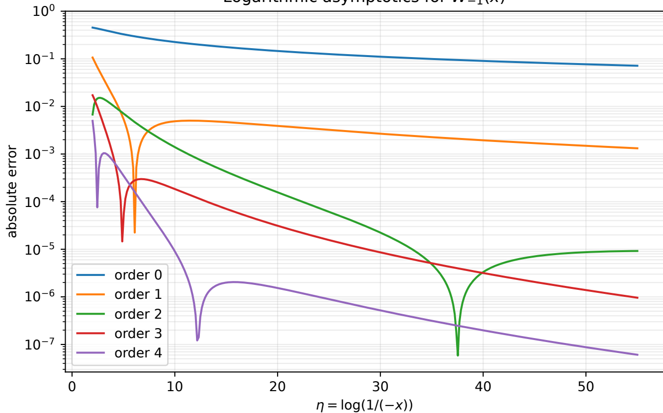
Logarithmic asymptotics for W_{-1}(x)
