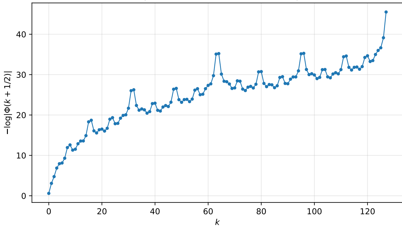
Decay of the half-lattice Fourier samples
