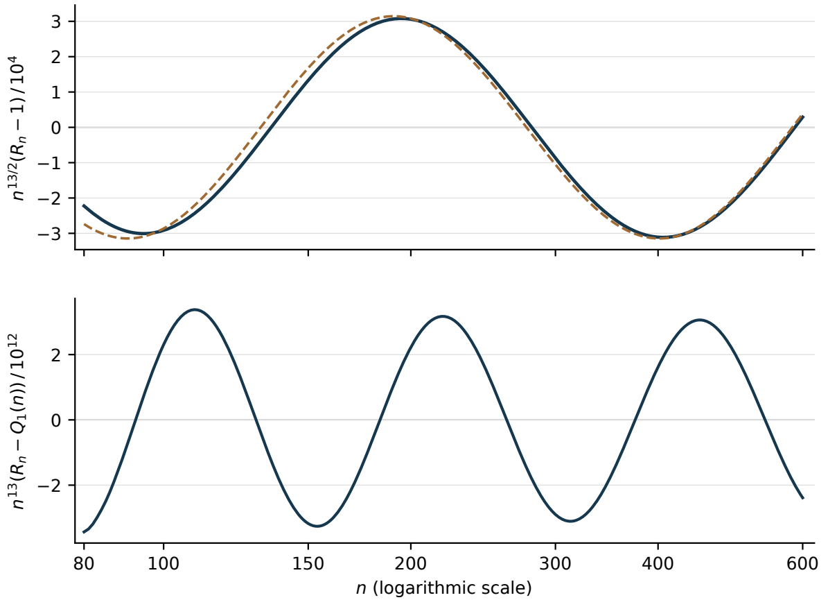
Figure 1: Exploratory illustration using exact counts for every integer 80 \leq n \leq 600 and the fitted constants in (10.1). The upper panel shows the logarithmically oscillating normalized discrepancy (solid) and its leading cosine (dashed). The lower panel scales the residual after the exact first Gamma-ratio correction by n^{13} . The figure illustrates the proven orders but does not certify the constants or a uniform numerical bound.
