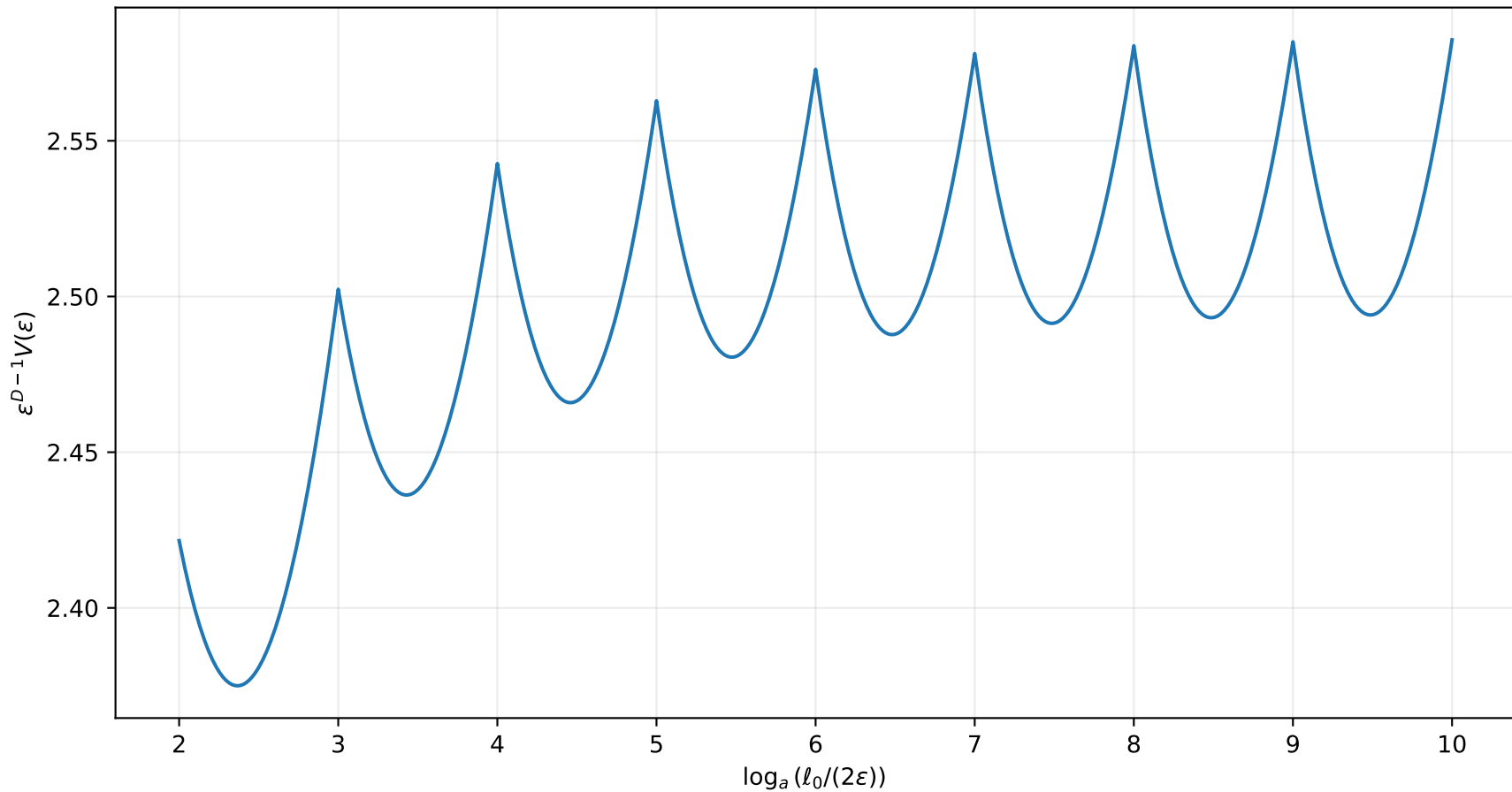
Exact lattice tube oscillation for the singular set, a = 3
